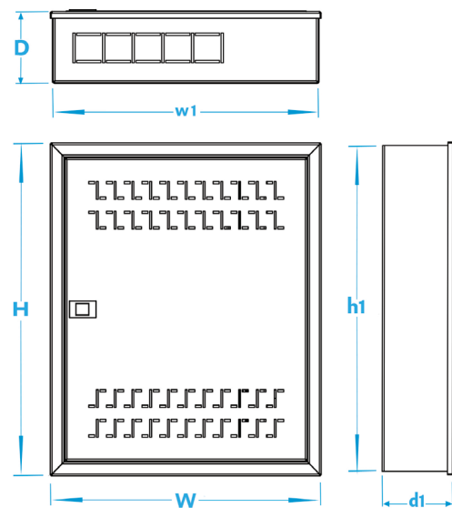
Wall Mounted
