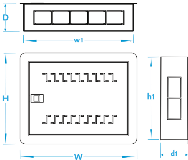
Flush Mounted
